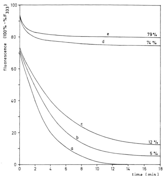
Fig. 7. Influence of NaCl on rate and extent of dissociation at 25 °C. Decay of fluorescence intensity at 333 nm (excitation at 290 nm) during dissociation of 0.1 mg/ml glucose dehydrogenase in 50 mM glycine-Tris buffer (pH 9): (a) 0 and 10 mM NaCl; (b) 50 mM NaCl; (c) 100 mM NaCl; (d) 500 mM NaCl; (e) 500 mM NaCl, protein concentration raised to 0.6 mg/ml. The intensity change for complete dissociation in the absence of NaCl (curve a) was set as 100%.
